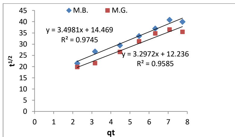
Figure 11. Intra particle diffusion plot for removal of dyes from binary mixture by C.media
