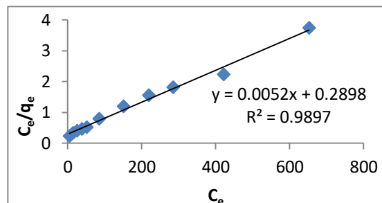
Figure 8. Langmuir model for removal of M.B. from binary solution by C. media
