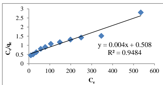
Figure 7. Langmuir model for removal of M.G. from binary solution by C. media
