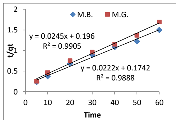
Figure 10. Pseudo Sec-order model for removal of dyes from binary mixture by C. media
