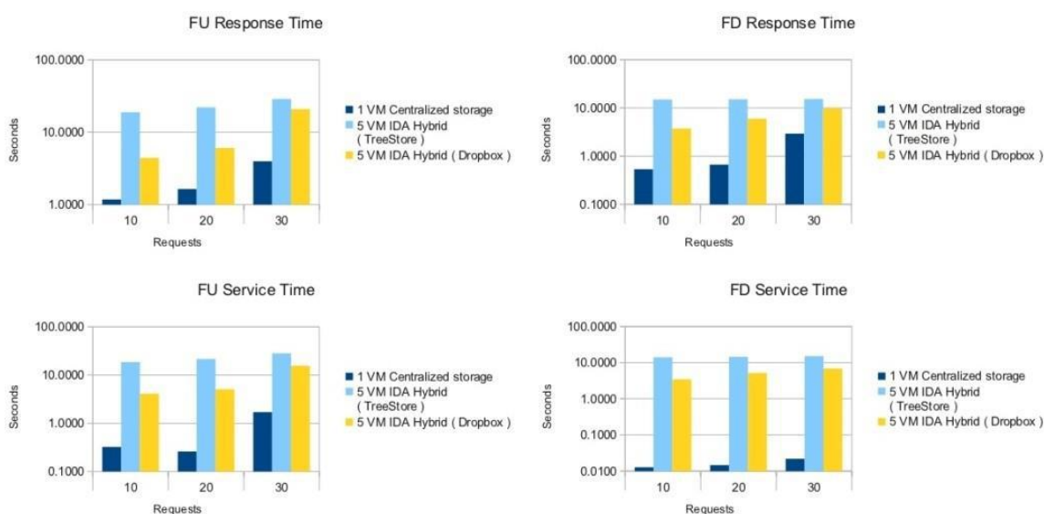
Figure 4: Average Response and Service Time for File Uploading (FU) and Downloading (FD) in the Evaluation of the Hybrid Cloud
