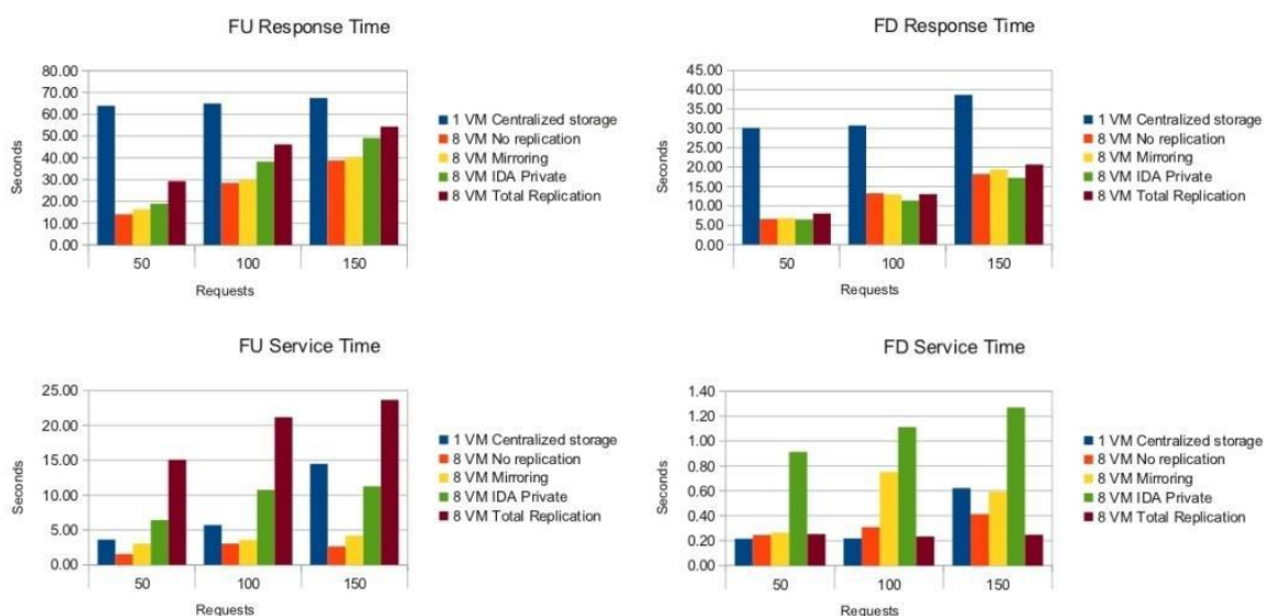
Figure 3: Average Response and Service Time for File Uploading (FU) and Downloading (FD) using Different Replication Techniques in a Private Cloud Environment
