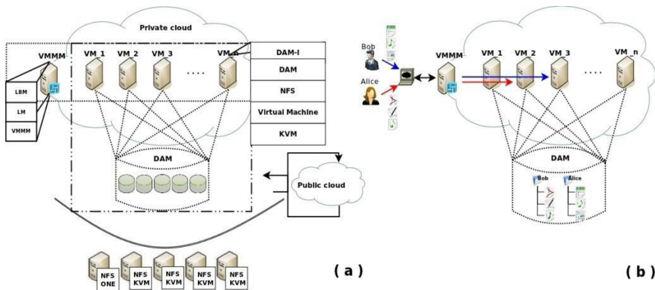
Figure 1: Main Components of the Cloud Storage Architecture
